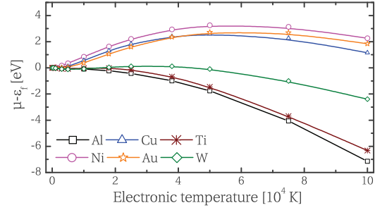
FIG. 5. (Color online) Electronic chemical potential evolution with the electronic temperature for all studied metals.
