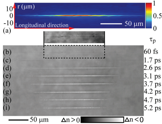
FIG. 1. (a) Longitudinal profile of the experimentally generated Bessel beams in air. (b)–(i) PCM images (side-view) of single-shot structures machined inside fused silica using E = 4.1 \mu\text{J}/\text{pulse} and \tau_p = 60 \text{ fs} - 5.2 \text{ ps} revealing morphological changes corresponding to Type I and II regimes. Inset to (b) shows the portion of the image with low contrast for visibility. \Delta n represents the laser induced refractive index change of the material.
