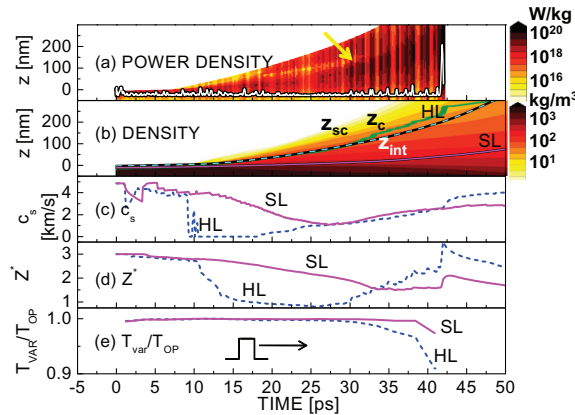
Figure 4. (a) OP temporal shape superimposed on the instant values of absorbed power density given on a logarithmic scale ( Q_L ). An arrow indicates the absorption frontier (see z_{sc} below). (b) Density dynamics of excited matter for OP. The HL, SL evolutions are given (dashed, solid, respectively). The continuous line ( z_c ) represents the critical electron density border (at 800 nm), with z_{sc} being layers with subcritical electronic density and z_{int} layers with high electronic density. (c) The evolution of the speed of sound c_s for HL and SL. (d) The ionization dynamics for HL and SL. (e) Effect of canceling particular peaks in the OP sequence on the achieved maximal temperature.
