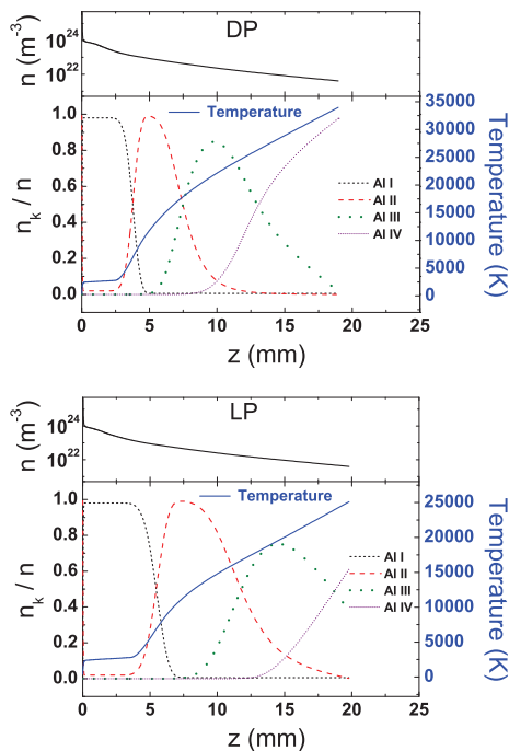
FIG. 8. (Color online) Spatial profiles of density n(z) , temperature T(z) , and species proportions n_k/n of atoms Al-I to Al-IV simulated at t=250 \text{ ns} after the laser impact for temporally tailored incident DP and LP ( z=0 at the surface). The incident fluence is 5.8 \text{ J/cm}^2 .
