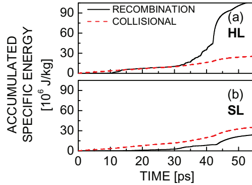
Figure 5. Energy deposition by collisional and recombination mechanisms for (a) HL and (b) SL. Solid line, \int_0^t Q_{\text{rec}}(t') dt' , dotted line, \int_0^t Q_{e-i}(t') dt' .
