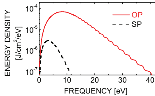
Figure 7. Integrated spectral energy density emitted by the electrons for SP and OP, including contributions from all excited layers within the first 100 ps. A significantly increasing magnitude and a shift towards higher energies for the OP-induced spectrum can be observed.
