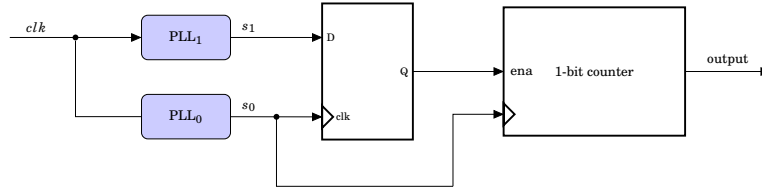
Figure 4.5: PLL-TRNG with two PLLs in parallel.
