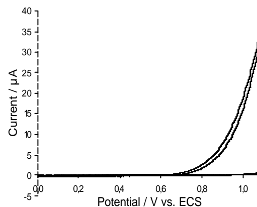
Fig.1a Cyclic Voltammograms of DLCs films with different ratio \text{sp}^3/\text{sp}^2 carbon hybridization in 40 mM PB solution, pH 7.4 and with 5 mM \text{H}_2\text{O}_2 in PB.
