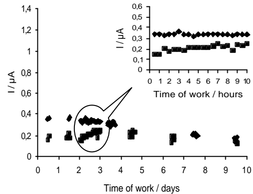
Fig.4 Operational and storage stability of SiCar1 (?) and SiCNi5% (i) biosensors for 0.5 mM glucose concentration.
