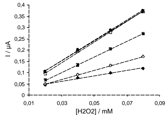
Fig.2 Hydrogen peroxide calibrations curves for SiCar1 ( ? ), SiCar2 ( ? ), SiCar3 ( ◊ ), SiCNi2% ( ◊ ), SiCNi5% ( ◻ ) and W-containing DLN ( • ) for successive additions of 0.02 mM H_2O_2 in 40 mM PB, pH 7.4.
