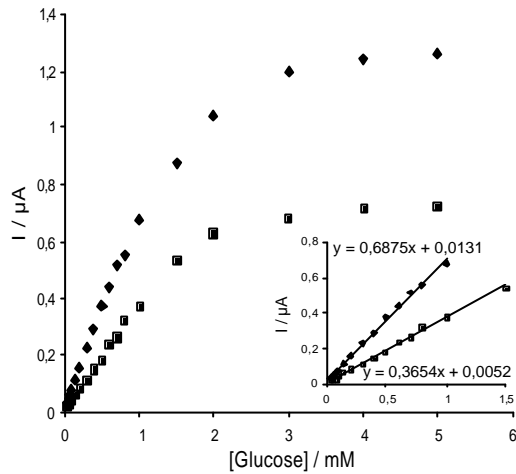
Fig. 3 Glucose Calibration curves for SiCar 1 (?) and SiCNi 5% (i) electrode for successive additions of glucose in 40 mM PB, pH 7.4.
