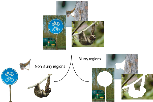
Fig. 2. Blur identification
