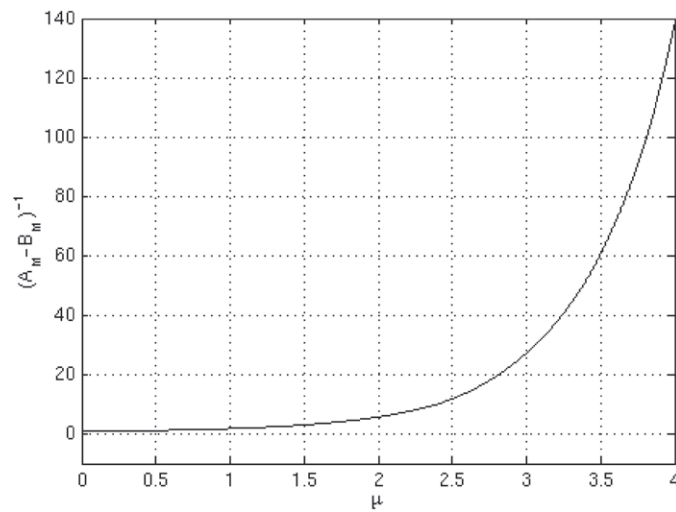
Figure 6. Plot of 1/(A_M - B_M) as a function of \mu for M = 40 . This quantity is an upper bound on how errors in the DBP result due to data noise are amplified through the inversion of (30), as explained by equations (40) and (45).
