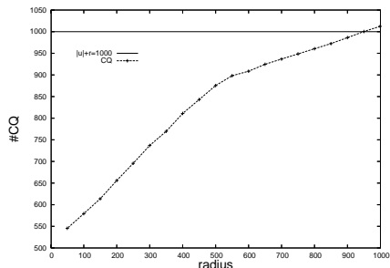
Fig. 1. Number of CQ needed to identify a ball B_r(o) when |o| + r = 1000 . For each r , we compute the average over 100 balls.
