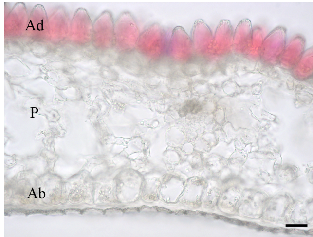
Figure 1. Hand-made cross-section of Rosa x hybrida petal; Ad, adaxial epidermis; Ab, abaxial epidermis; P, spongy parenchyma. Bar, 20 \mu\text{m} .
