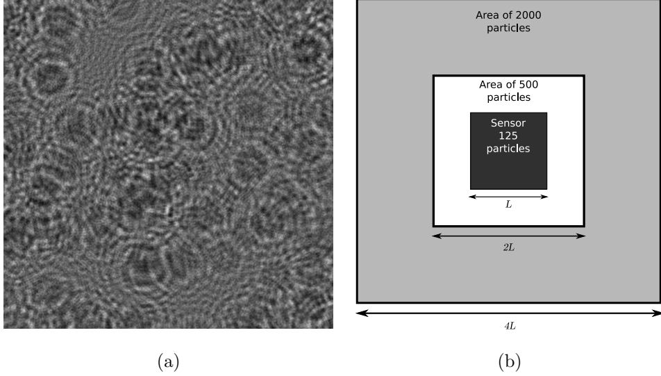
Figure 8. (a) Example of a hologram simulation ( 1024 \times 1024 ) made with 2000 particles (diameter of 100\mu m ) spread throughout a volume of 27.44 \times 27.44 \times 50mm located at z_0 = 250mm . The pixel size is 6.7 \times 6.7\mu m and the laser wavelength is 0.532\mu m . The hologram is coded on 8 bits depth. (b) Illustration of the distribution of particles throughout the volume: 125 particles are located on the sensor (dark gray area of width L ), 500 out-of-field particles are located on the white area (4 times the sensor area), and 1500 particles are located around the white area (in the light gray part) which corresponds to the background noise.
