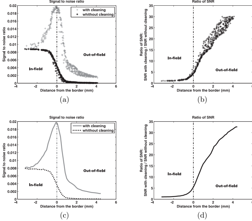
Figure 9. (a) Evolution of the SNR in the hologram during the detection of the particle. The curve plotted with \times shows the evolution for an approach without particle cleaning. The curve plotted with + shows the evolution of the SNR for an approach with an iterative particle cleaning (described in section 3.3). (c) represents the mean curve of (a) over 10 simulations. (b) Ratio of the SNR of the iterative cleaning approach to the SNR without cleaning. (d) represents the mean curve of (b) over 10 simulations. The vertical dash-dotted line on all figures represents the transition between in-field and out-of-field particles.
