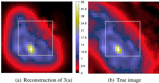
Figure 4: Image ( 32 \times 32 ) at \lambda = 3967.4 \text{ \AA} with extrapolation
