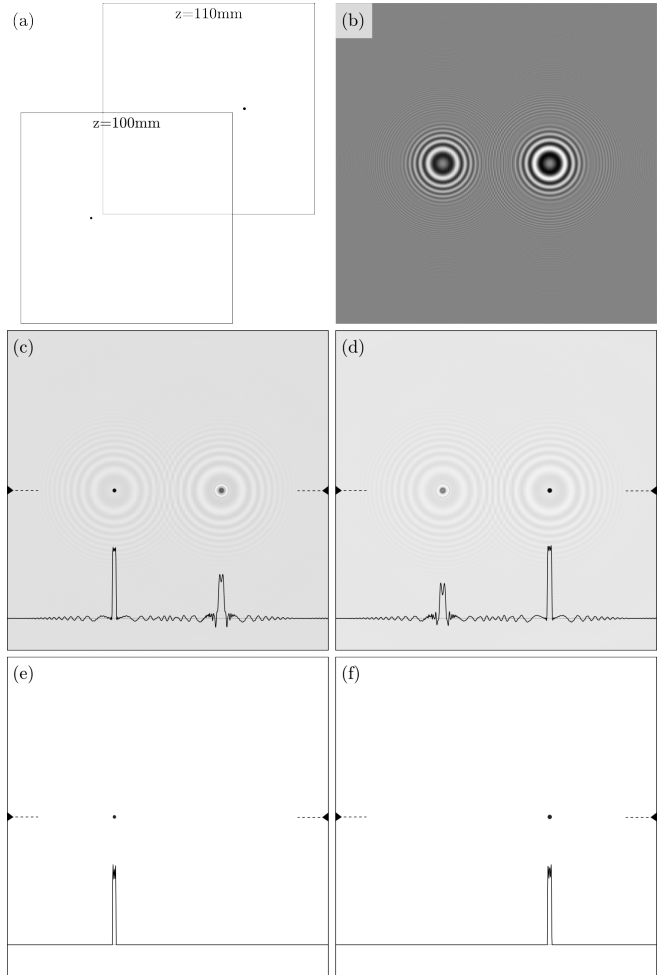
Fig. 1. Reconstruction of a simulated hologram (b) of two opaque disks located respectively at 100mm and 110mm from the hologram plane (a): (c-d) conventional reconstruction \hat{\vartheta}^{\text{adj}} ; (e-f) sparse reconstruction \hat{\vartheta}^{\text{sparse}} (200 iterations). Superimposed is the transmittance profile over the line between \blacktriangleright \blacktriangleleft signs.
