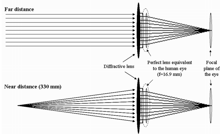
Fig. 3. Optical system used in the simulation of the MTF with Zemax® for near and far objects.
