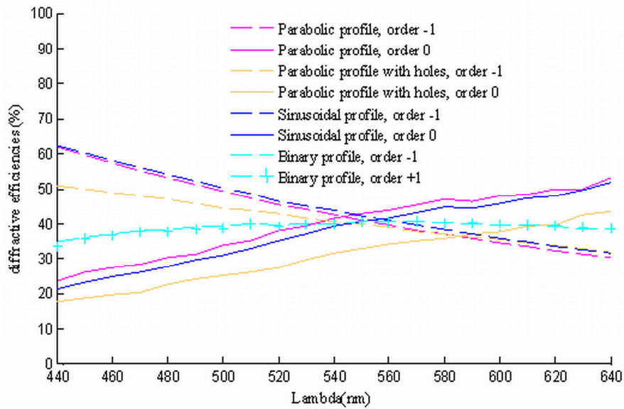
Fig. 5. Variations of the diffractive efficiencies versus \lambda
