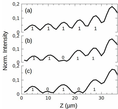
Fig. 3. Calculated intensity profiles along the optical axis z just before the main focus for different wavefront modulations controlling the dots local mapping. (a) no phase modulation yielding "11111" sequence. (b) and (c) various modulations yielding "11011" and "10101".
