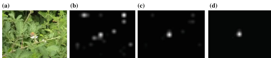
Fig. 16 Example of saliency map computed for a frame without face. When the weight of C_F = 3/8 and w_i = center-surround filter, the stationary saliency map better detects the butterfly at the center of the image. a Original frame. b Stationary saliency map with a weight of 0
