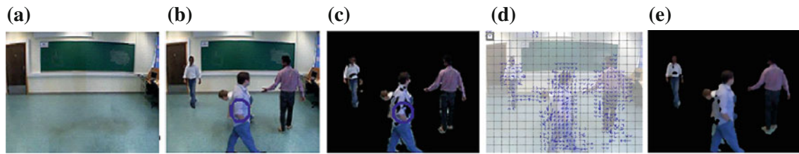
Fig. 7 Foreground extraction with or without taking into account the motion vector field. a Background image. b Current frame image. c Foreground objects. d #173 motion vector. e Improved foreground
