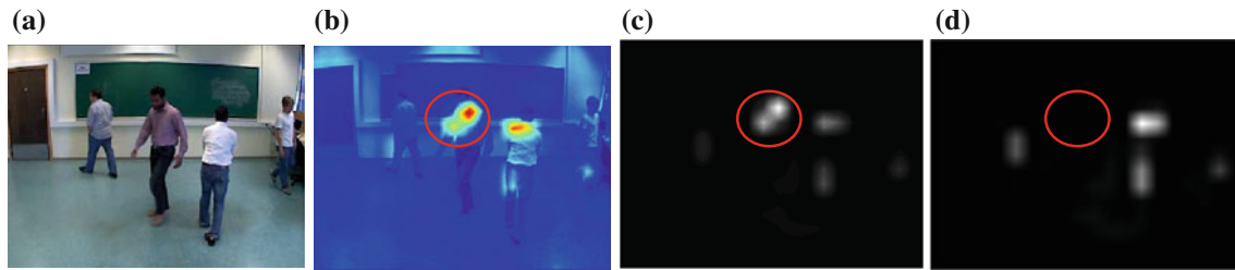
Fig. 9 Saliency map computed with different weights for merging C_F with other features. When the weight of C_F = 0 that means that we do not take into account the face feature C_F in Eq. (9). The main difference between these saliency maps is surrounded in red.
