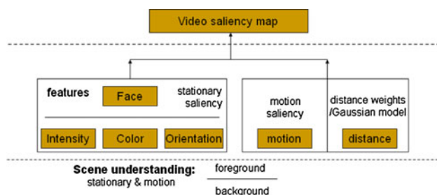
Fig. 1 Synopsis of the spatiotemporal saliency model proposed
