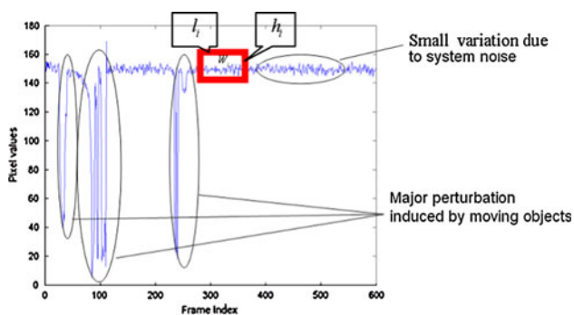
Fig. 3 Pixels intensity variation at the center of the dark circle
