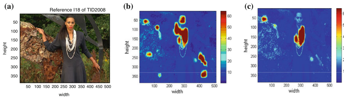
Fig. 10 Saliency region from stationary model and Itti's model. a I18 image in TID2008. b Saliency map from stationary model. c Saliency map from Itti's model
