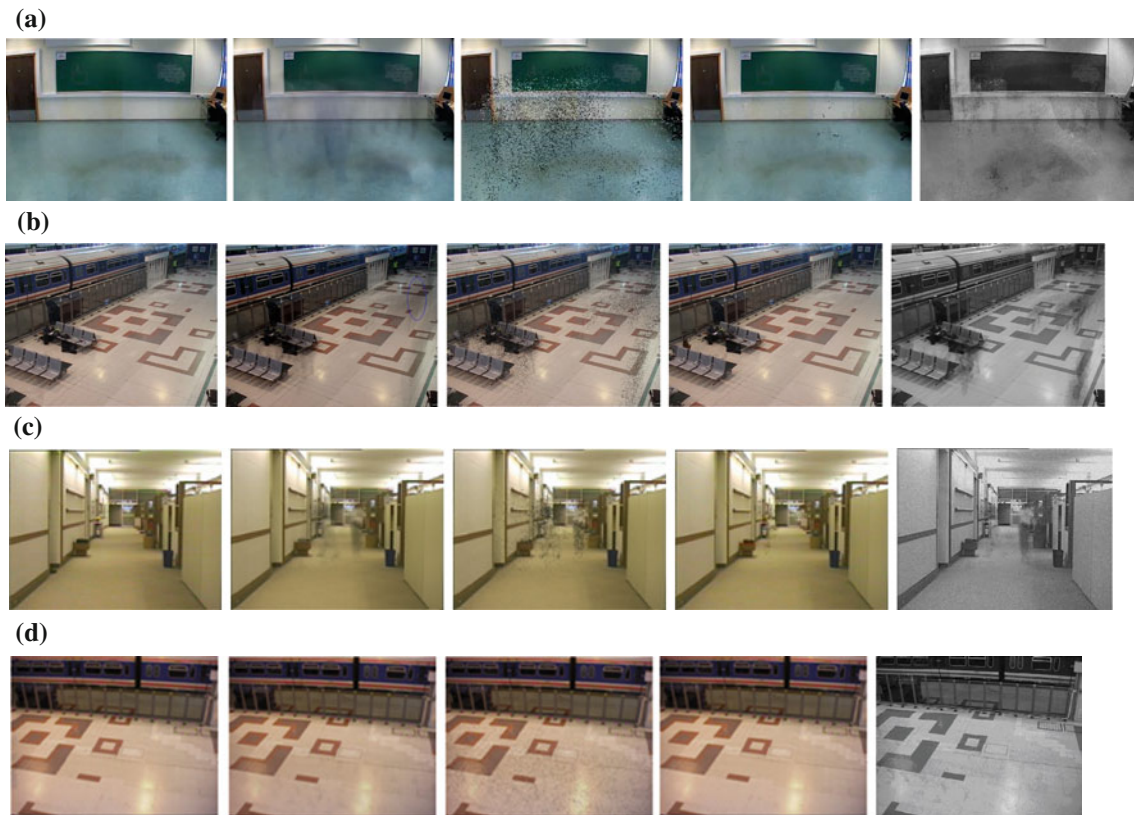
Fig. 6 Comparison of generated backgrounds: (1st column) Ideal background, (2nd column) mean value, (3rd column) mean shift (4th column) with our method, and (5th column) with Mixture of Gaussians (MOG) [28]. a Background generation: example 1. b Background generation: example 2. c Background generation: example 3. d Background generation: example 4
