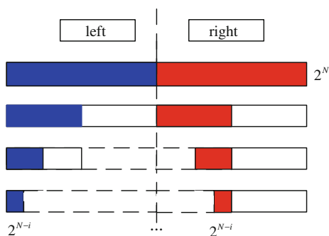
Fig. 4 Binary tree search process
