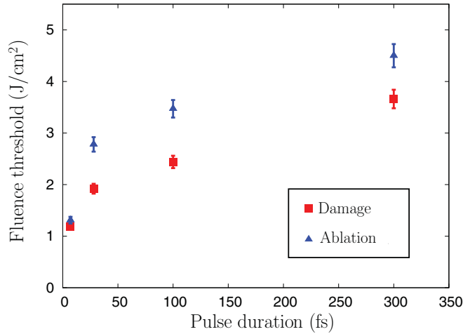
FIG. 2. (Color online) Damage and ablation fluence thresholds as a function of laser pulse duration. The error bars correspond to shot-to-shot energy fluctuations measured to be about 10% for all pulse durations.
