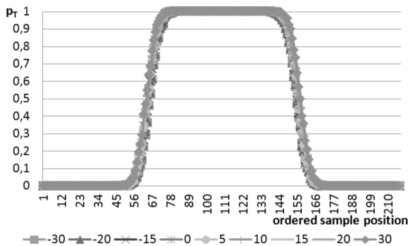
Fig. 6. Probability chart for samples of a jitter influenced clock signal CLJ accumulated during N = 1000 of T_Q periods for PLL-TRNG with PLL Configuration B with K_D = 217 for temperatures in range T = (-30^\circ\text{C}, +30^\circ\text{C}) .
