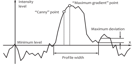
Fig. 5. Width estimation of the edge gradient profile.
