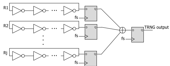
Fig. 1. RO-TRNG.
