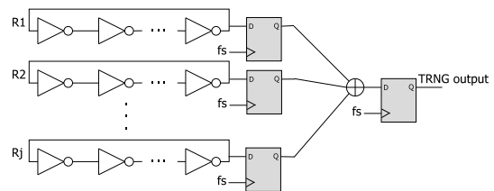
Fig. 1. RO-TRNG.
