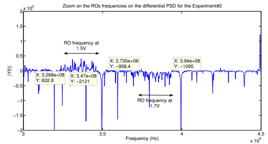
Fig. 7. Differential PSD of the Experiment #2 at the center of the chip
