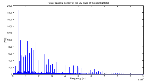
Fig. 4. Typical Power spectral density of the EM traces at a random location in the EM device map
