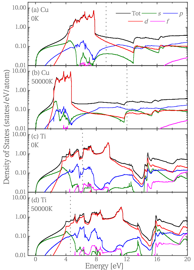
FIG. 4. (color online). Evolution of the total DOS and spdf -components of the DOS for Cu at 0K (a) and 5 \times 10^4\text{K} (b), and for Ti at 0K (c) and 5 \times 10^4\text{K} (d). Dashed lines correspond to Fermi levels.
