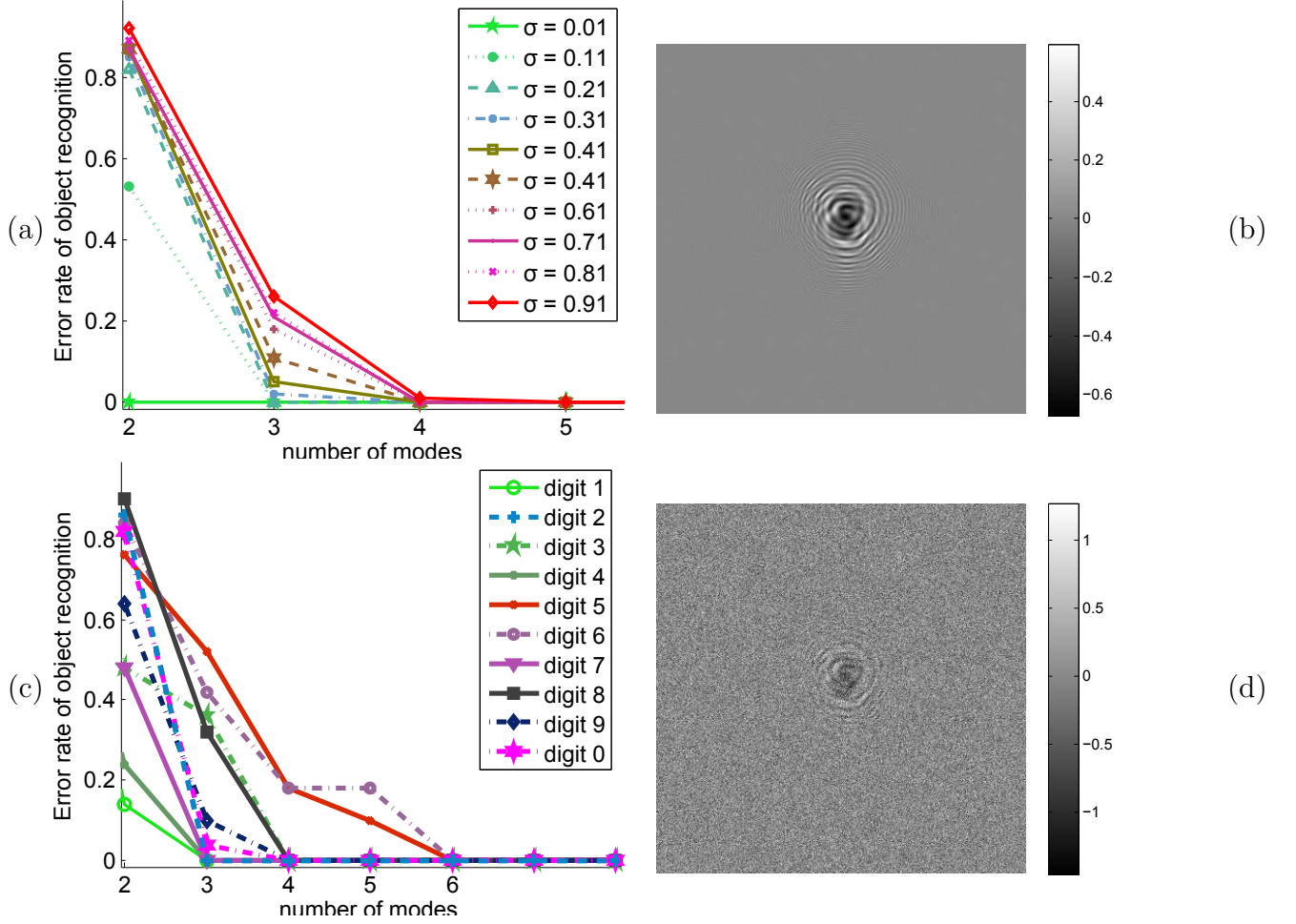
Fig. 5. Study of the error rate on object recognition for the toy problem of holograms of digits (see Sec. 4.A). (a) shows the error rates of object recognition for a '2' placed at 0.17m from the sensor. The curves show the error rate for different approximation ranks and different noise levels, (b) illustrates one hologram of 2 degraded by white Gaussian noise with \sigma = 0.01 , (c) plots the error rates representing the discriminating power of approximated dictionaries for a fixed level of noise resulting in a \text{SNR} \approx 3 , (d) illustrates one of the holograms of Sec. 4.A for object '2' placed at 0.17m from the sensor.
