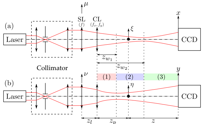
Fig. 1. (Color online) Experimental configuration for digital hologram recording with an astigmatic reference beam. (a) x, z view. (b) y, z view. SL: Spherical Lens, CL: Cylindrical Lens
