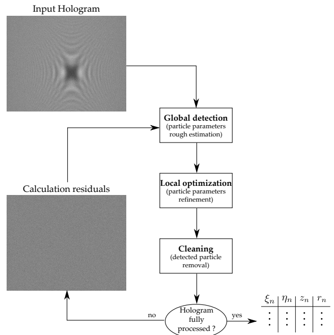
Fig. 4. Synoptics of the “inverse problems” approach algorithm.
