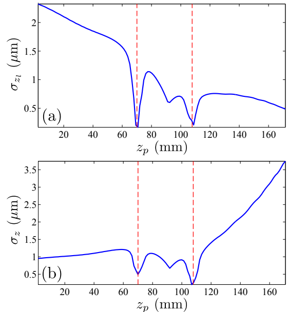
Fig. 5. (Color Online) Theoretical study of the evolution of (a) \sigma_{z_l} and (b) \sigma_z standard deviations versus the distance z_p between CL and the object. The experimental parameters are the same as in Section 2. Red dashed lines are associated with beam waist positions.
