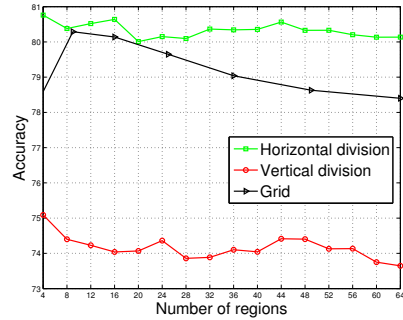
Figure 2: Classification accuracy versus number of local regions for the 15 Scenes dataset using pairwise matching and different partitioning schemes: grid, vertical divisions or horizontal ones.
