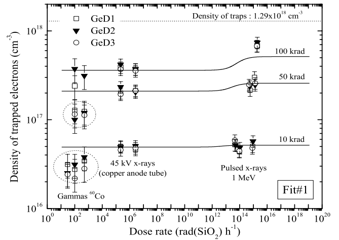
Fig. 9. Steady-state trap fillings in GeD1, GeD2 and GeD3 after 10, 50 and 100 krad doses. Symbols = data. Lines = computed projections for fit#1. TSL responses have been converted into absolute electron densities with N = 1.29 \times 10^{18} \text{ cm}^{-3} . Dose rates are calibrated with \beta = 10^{-10} \text{ cm}^3 \text{ s}^{-1} .
