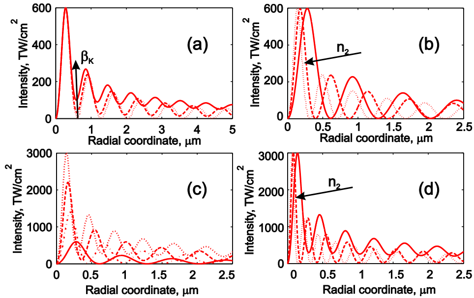
Fig. 5. Comparison of the stationary NBV when the NLL coefficient is changed. (a) \beta_K is changed (from 4.7 \times 10^{-27} to 42.3 \times 10^{-27} \text{cm}^3/\text{W}^2 ). The black arrow represents increasing \beta_K values while n_2 is fixed at 3.45 \times 10^{-16} . (b,d) The nonlinear refractive index n_2 is changed (from 3.45 \times 10^{-16} to 17.25 \times 10^{-16} \text{cm}^2/\text{W} ) and \beta_K = 4.7 \times 10^{-27} \text{cm}^3/\text{W}^2 . The black arrow represents increasing nonlinear index coefficients. The higher maximum intensity in case (d) induces a stronger influence of NLL compared to case (b). (c) \beta_K and n_2 coefficients are fixed, while leaving free the maximum intensity. For all figures, the Bessel beam angle is \theta = 16.4^\circ .
