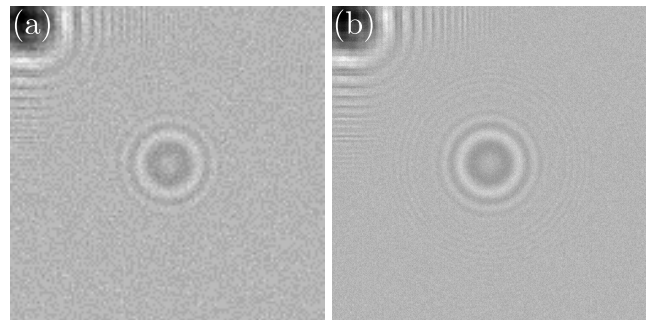
Fig. 3. Illustration of the super-resolution by IP approach with joint optimization. (a) Simulated low resolution hologram ; a Gaussian white noise has been added so that the SNR of hologram is 5. The image area represents 128x128 pixels. (b) Hologram super-resolved by a factor 4 using the proposed method (given for illustration purposes).
