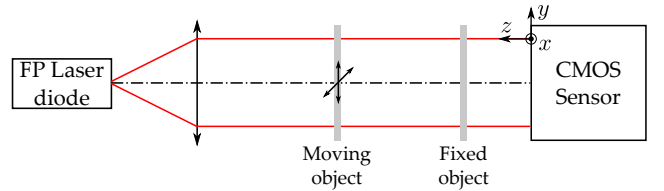
Fig. 2. (Color online) Experimental configuration for super-resolution of particle holograms.
