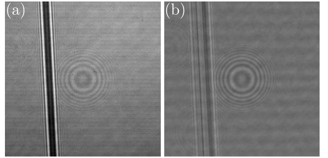
Fig. 4. Illustration of the super-resolution by IP approach with joint optimization. (a) Acquired low resolution hologram. The original image was cropped to 320x320 pixels. (b) Hologram super-resolved by a factor of 4 using the proposed method (given for illustration purposes).
