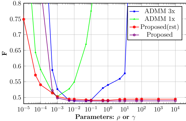
Fig. 2: Influence of the penalty parameters on the convergence speed: function cost at 1500 FFT evaluations vs. penalty parameters, \rho for ADMM 3x ( \nu and \gamma at possible best values), and \gamma for remaining two methods.
