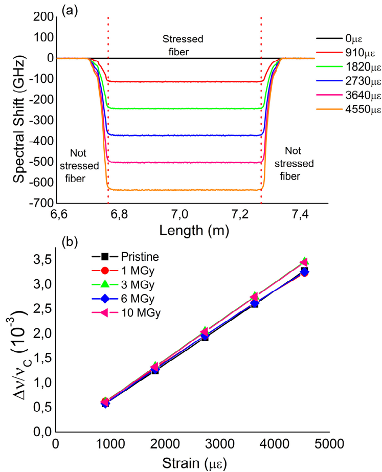
Fig. 4. (a) Example of Rayleigh spectral shift in SMF 28 sample as a function of fiber length at different applied strains from 0\mu\text{e} (reference trace) up to 4550\mu\text{e} and (b) measured Rayleigh spectral shift dependence on strain for SMF28 non-irradiated and irradiated samples at 1MGy, 3MGy, 6MGy and 10MGy shown for one point for each fiber in the considered range chosen to calculate C_e .
