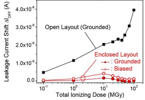
Fig. 3. Leakage current shifts \Delta I_{OFF} vs TID in Open Layout Transistors (OLT, black squares) and Enclosed Layout Transistors either grounded (ELT, filled red circles) or biased (ELT, open red circles) during irradiation.
