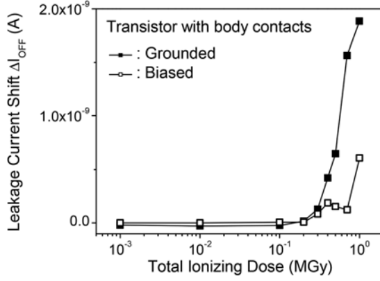
Fig. 4. Leakage current I_{\text{OFF}} shifts induced after 1 MGy on a Body Contacted transistor either grounded (filled squares) or biased (open squares) during irradiation.
