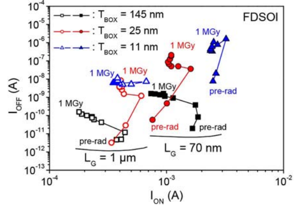
Fig. 5. I_{\text{ON}} - I_{\text{OFF}} characteristics as a function of TID on FDSOI transistors processed on SOI substrates with a BOX thickness T_{\text{BOX}} = 145 nm (black squares), T_{\text{BOX}} = 25 nm (red circles) and T_{\text{BOX}} = 11 nm (blue triangles). Transistors with both a short gate length ( L_G = 70 nm, filled symbols) and a long gate length ( L_G = 1 \mu\text{m} , open symbols) are plotted for each SOI substrate option. Devices are grounded during irradiation.
