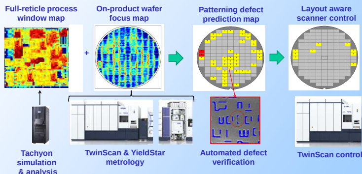
Holistic lithography concept for patterning defect prediction and layout aware scanner control
