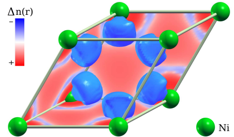
FIG. 1. (Color online) Representation of the electronic density changes from T_e = 0 K to T_e = 2.5 \times 10^4 K, for a primitive cell of FCC Ni. In blue, isosurface of electronic density loss. In red, mapping along basal planes of the electronic density gain.
