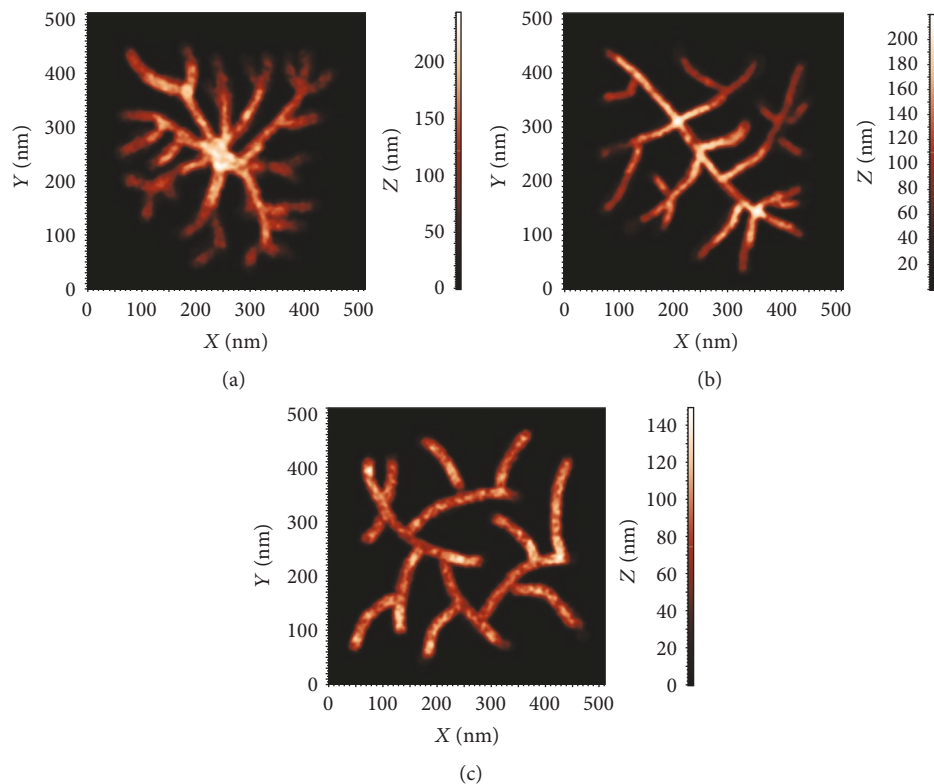
FIGURE 6: Three different morphologies of the obtained fractal aggregates: (a) “star” configuration; (b) “leaf” configuration; and (c) “branches” configuration.
