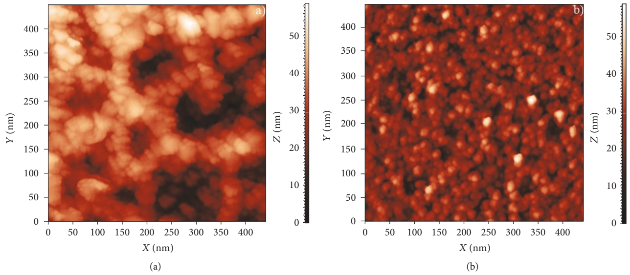
FIGURE 2: AFM images of gold (a) and silver (b) particle deposited on the substrate. Here, laser power is 2.5 W; the structures are formed for 25 laser passages with the scanning speed of 1.2 mm/s.
