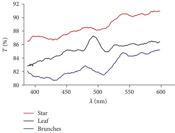
FIGURE 8: Measured transition spectra of fractal aggregate shown in Figure 4.
