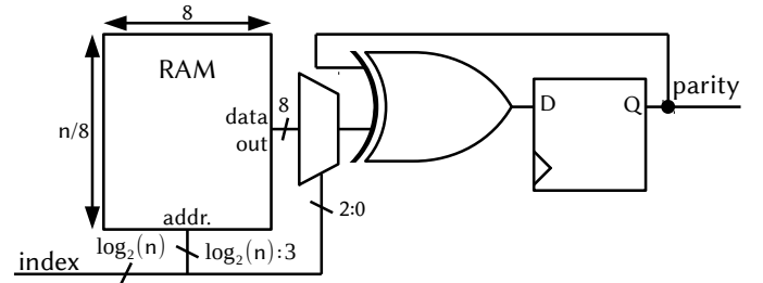
Fig. 12: Hardware architecture of the parity computation module where the PUF response is stored in RAM
