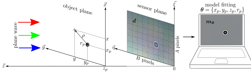
Fig. 1. Lensless color microscopy setup.
