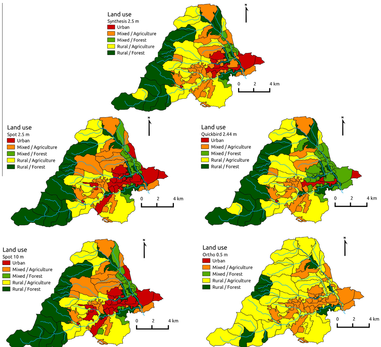
Fig. 3. Model HRUs and reaches and land use classification for Synthesis 2008, Spot 2008 (2.5 m and 10 m), Quickbird 2008 and Ortho 2008 land use maps.
