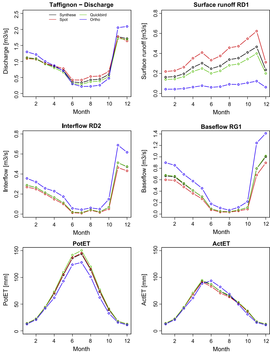
Fig. 5. Comparison of the interannual monthly mean simulated total discharge and runoff components, mean annual potential evapotranspiration (PotET) and mean annual actual evapotranspiration (ActET) for the maps Synthese (black), Spot 2.5 (red), Quickbird (green) and Ortho (blue) at the catchment outlet (Taffignon station). (For interpretation of the references to colour in this figure legend, the reader is referred to the web version of this article.)
