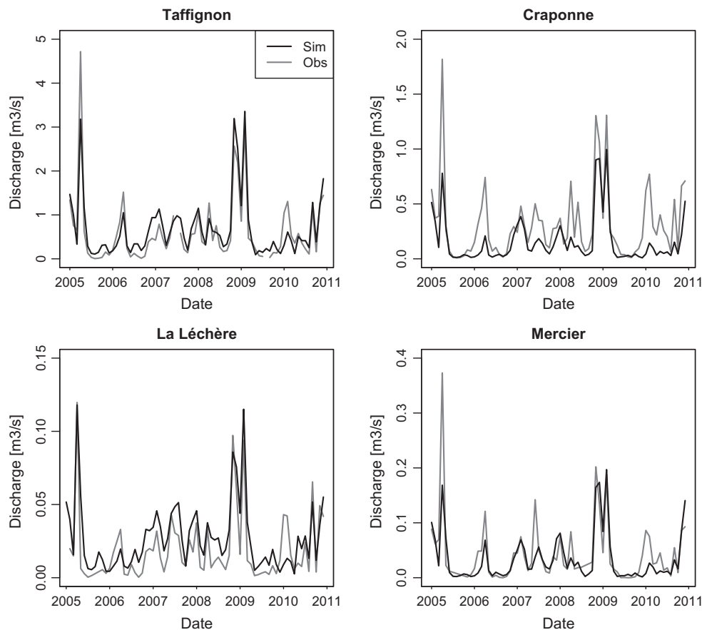
Fig. 4. Model evaluation: simulated (black) and observed (gray) monthly mean discharge values during the 2005–2010 period for the outlet station (Taffignon) and the intermediate stations Craponne, La Léchère, and Mercier.
