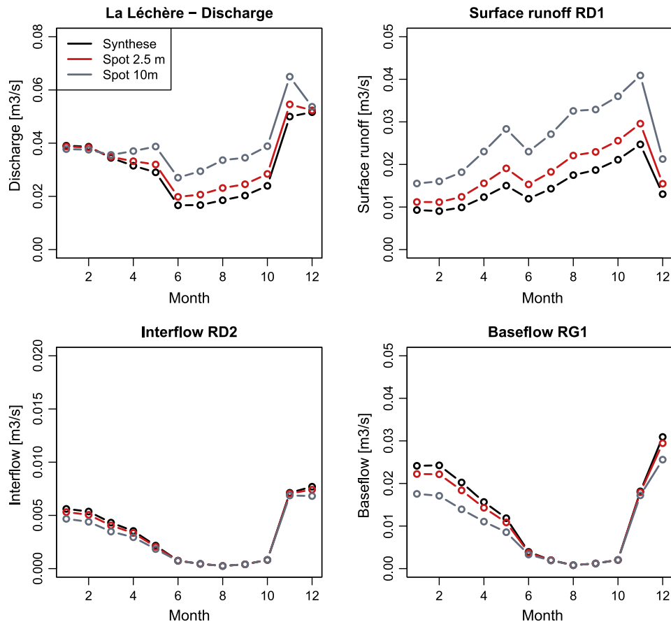
Fig. 7. Comparison of the interannual monthly mean simulated total discharge and runoff components for the maps Synthèse (black), Spot 2.5 (red), and Spot 10 (gray) at the La Léchère intermediate station. (For interpretation of the references to colour in this figure legend, the reader is referred to the web version of this article.)
