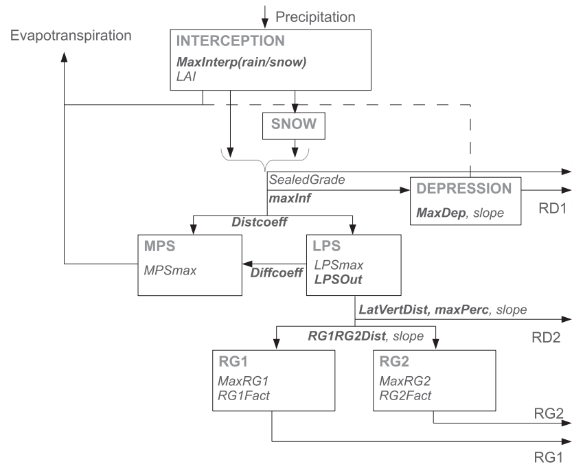
Fig. 2. Concept of the J2000 model showing the storages, the input and output flows for each HRU and the main parameters (italic). Parameters indicated in bold are lumped (1 value for the whole catchment), whereas the other parameters are distributed. J2000 provides also multiplicative lumped calibration parameters for each of the HRU outputs (RD1, RD2, RG1, RG2) and for the channel routing. These parameters were not used in this study and are thus not represented here.
