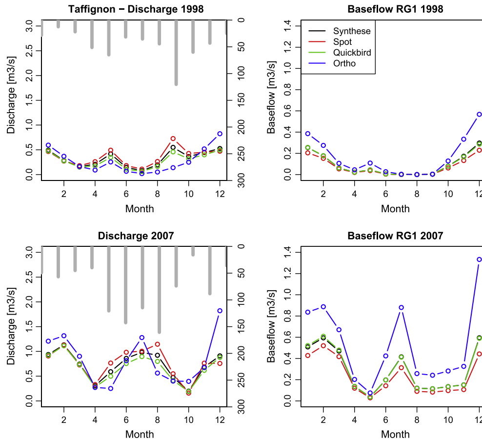
Fig. 6. Comparison of the monthly mean simulated total discharges and base flows for dry year 1998 (top) and wet year 2007 (bottom) for the maps Synthese (black), Spot 2.5 (red), Quickbird (green) and Ortho (blue) at the catchment outlet (Taffignon station). (For interpretation of the references to colour in this figure legend, the reader is referred to the web version of this article.)
