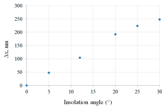
Figure 2. Lateral shift of the maximum intensity of the nanojet inside the \text{TiO}_2 film versus exposure angle.
