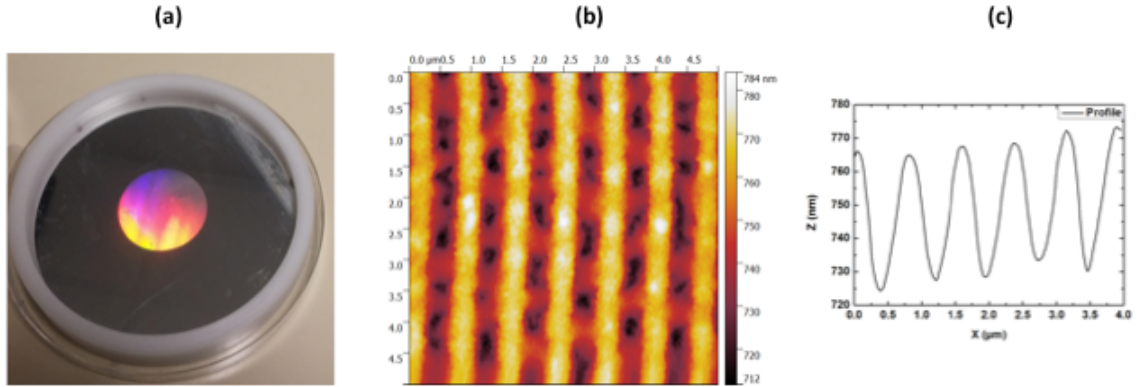
Figure 4. Grating: (a) Photograph, (b) 2D AFM image, (c) AFM profile.
