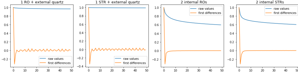
Figure 9: Autocorrelations of raw counter values and their first differences in the four hardware configurations. At lag 0, the correlation is by definition always equal to 1.
