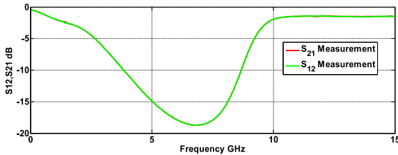
Fig. 6. Transmission S -parameters in the demagnetized state.
