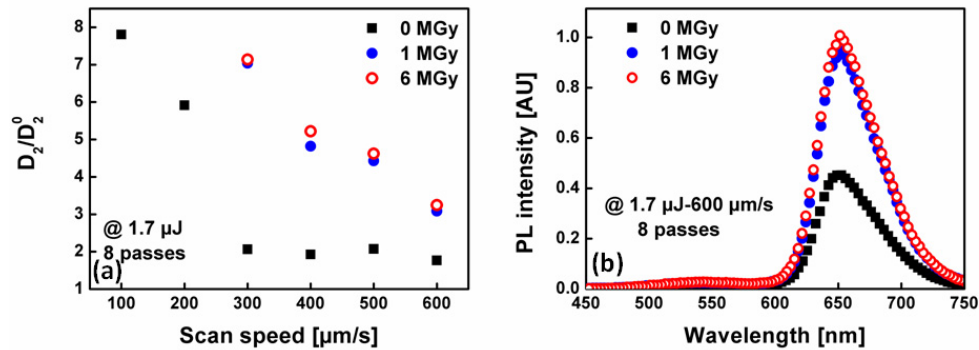
Fig. 5. (a) Relative D_2 areas normalized to the D_2^0 area (before X-ray treatment) at the maximum pulse energy of 1.7 \mu\text{J} as a function of the scan velocity for different accumulated doses. (b) PL measurements made in three waveguides written in a same condition (i.e. 1.7 \mu\text{J} -600 \mu\text{m/s} ) but in the different pre-irradiated samples.
