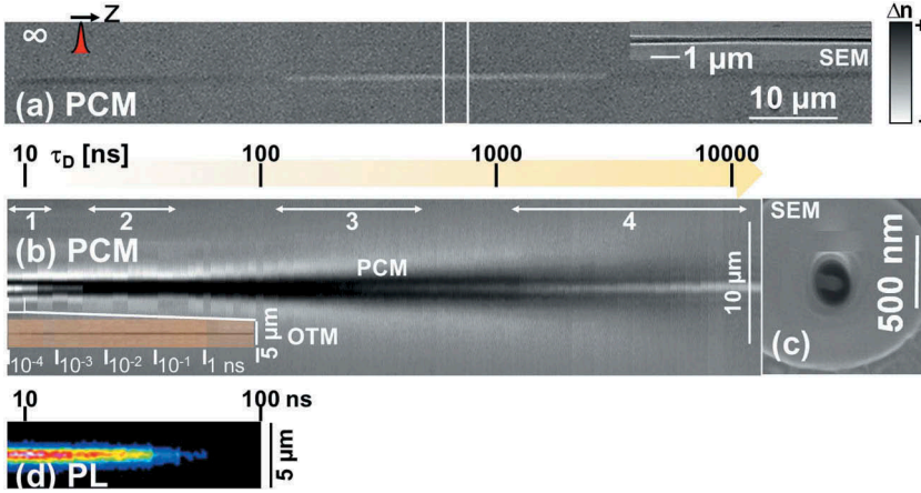
Figure 5. Dynamics of void generation under Bessel illumination. (a) Single shot ultrashort (50 fs) Bessel-induced negative index changes in bulk fused silica in tight focusing conditions ( \theta_{\text{glass}} \simeq 15^\circ ). The inset shows the interior of the structure in scanning electron microscopy. (b) Time-resolved sequence of phase contrast images of the excitation area over the entire relaxation cycle. The domain marked in (a) is chosen to reveal the time history by concatenating domain images at different time moments. Negative and positive phase shifts indicate: a long-living carrier plasma phase (1), a subsequent high index phase (2), heat diffusion (3), and the opening of the void (4). Time is indicated on a logarithmic scale. The inset shows optical transmission images with the absorptive signature of the carrier plasma. (c) The final transverse section of the void is given. (d) Photoluminescence (Bremsstrahlung) of the plasma in the visible range, suggesting an excited hot phase on tens of ns. Data from Ref [92].
