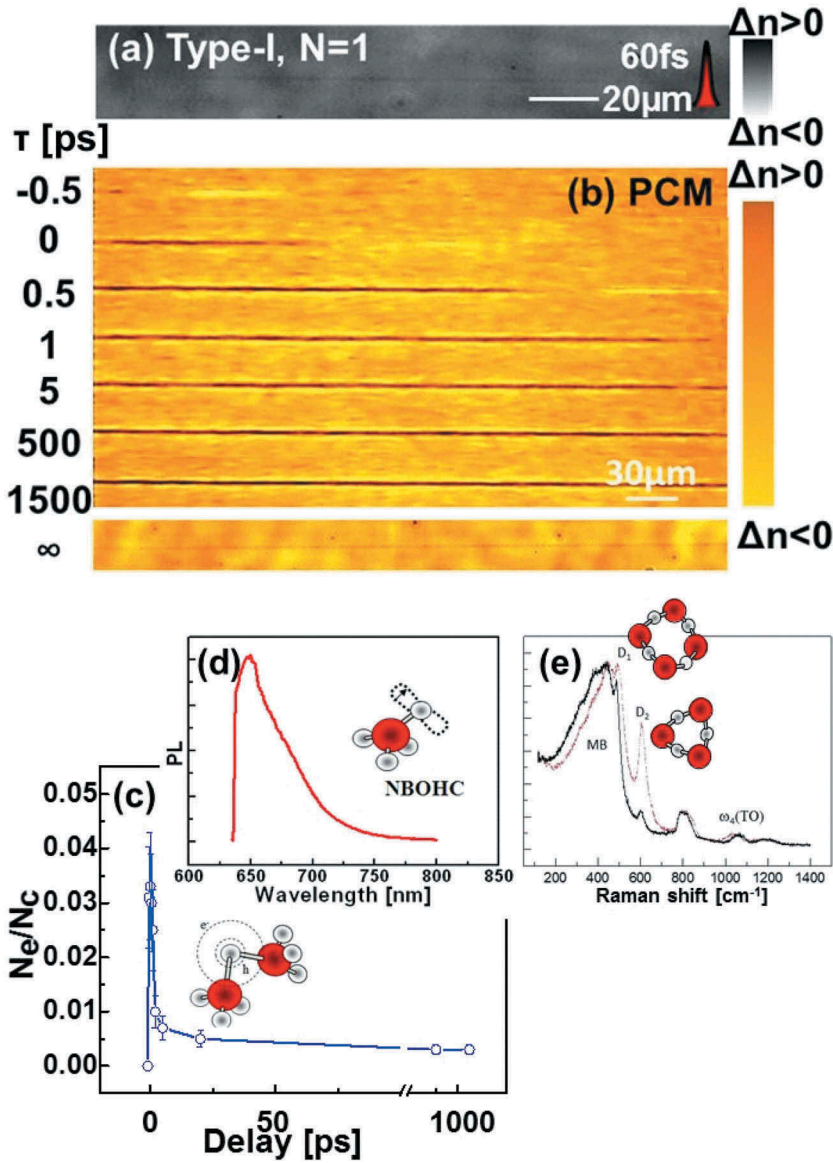
Figure 4. (a) Single shot Bessel-induced positive index changes in bulk fused silica with ultrashort pulses in conditions of moderate focusing ( \theta_{\text{glass}} \simeq 8^\circ ). The typical index contrast lies here below 10^{-4} . (b) Time-resolved sequence of phase contrast images of the excitation area showing the carrier evolution and relaxation. Carrier presence at the front is signaled by light colors (negative index change, due to electronic contribution to the dielectric function) while the subsequent positive index change following structural and electronic relaxation emerges rapidly in the wake of the electrons (dark colors). (c) Ultrafast carrier decay corresponding to type I photoinscription in fused silica. (d) Photoluminescence of NBOHC centers characteristic to type I change. (e) Typical Raman spectrum of type I densified regions in fused silica with representations of structural units for the D1 and D2 features. Data from Ref [46,85].
