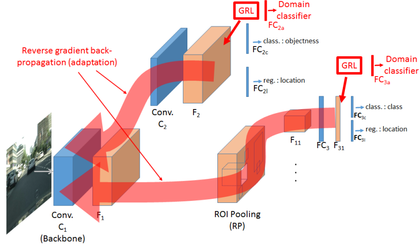
Fig. 3: Our domain adaptation for Faster R-CNN. See text for details.
