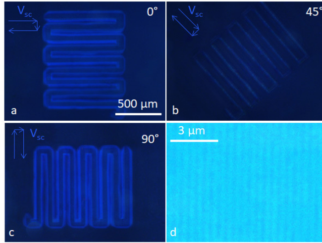
Figure B.7: Optical microimages of the structure obtained by laser scanning along Y-axis ( F=0.33 \text{ J/cm}^2 , N=1000 ) under polarized light. The orientation of polarization vector is shown to be parallel or orthogonal to the orientation of the periodical structures. The sample is located at different directions: a initial direction; b sample rotated for 45^\circ , c sample rotated for 90^\circ . d phase-contrast microimage.
