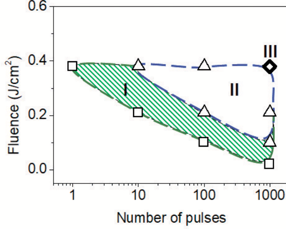
Figure 3: Laser processing regimes: zone I corresponds to the desirable interference pattern with \Lambda_1=540 nm recorded at F=0.15 J/cm 2 (Fig. 2b); zone II corresponds to the self-organized grooves (Fig. 2c); in the point 3, film destruction is observed (Fig. 2d).
