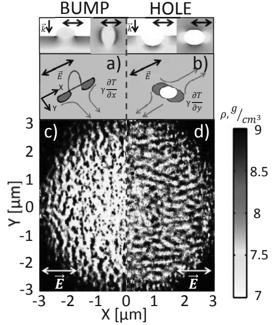
Figure 4: Mechanisms of convective instability development upon irradiation of surfaces with random (a) nanobumps and (b) nanoholes is illustrated. Upper images indicate the absorbed energy in the vicinity of a single nanofeature in propagation and transverse planes. Then, the direction of fluid flow from hot spots near bumps/holes is shown by red lines. The resulting density snapshots upon irradiation of surface with (c) nanobumps and (d) nanoholes of R = 5 nm with concentration C = 2\% indicate the formation of HSFL oriented (c) perpendicular or (d) parallel to laser polarization. Laser fluence is F = 0.25 J/cm 2 . The lattice density distributions are shown 100 ps after laser irradiation.
