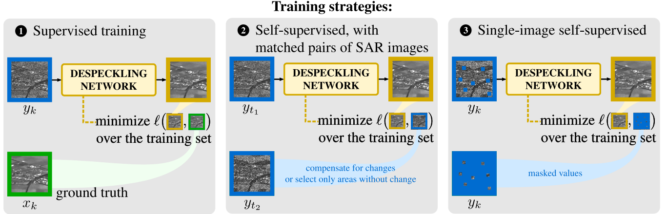
Fig. 1. Three training strategies have been explored in the literature: ① supervised training, using ground-truth images that match the speckled images provided as input to the network; ② self-supervised training, using co-registered pairs of SAR images captured at different dates; ③ self-supervised training, using single images and a masking strategy: the network is trained to correctly infer the masked pixels of the input image.
