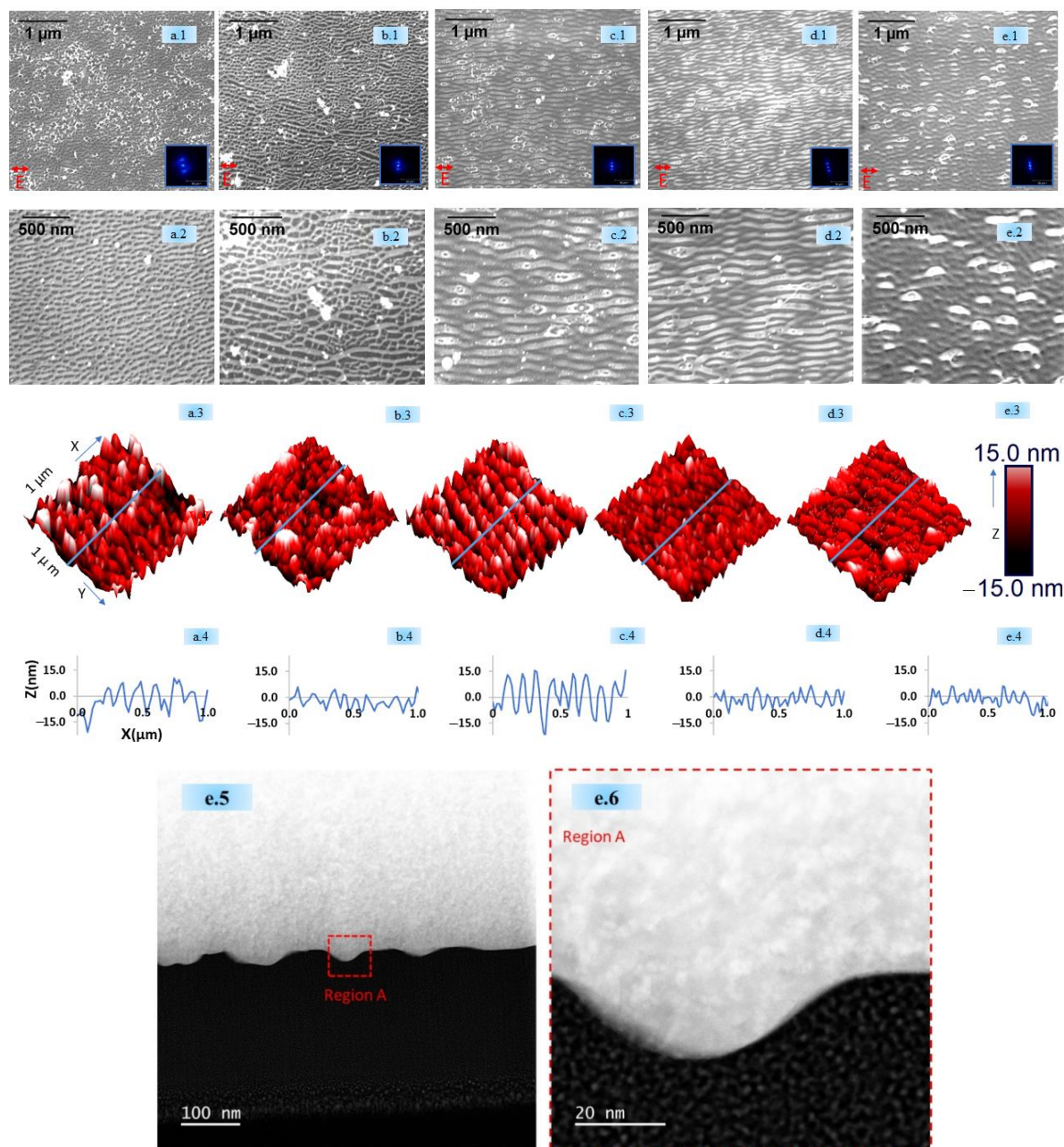
Figure 2. (i) Top (a.1–e.2) SEM images of HSFLs generated with no sputtering with FFT for (a.1,a.2) ambient, (b.1,b.2) air (10 mbar), (c.1,c.2) nitrogen (10 mbar), (d.1,d.2) argon (10 mbar), and (e.1,e.2) vacuum ( 10^{-7} mbar). (ii) Middle (a.3–e.3) AFM images ( 1 \times 1 \mu\text{m} area) for (a.3) ambient, (b.3) air (10 mbar), (c.3) nitrogen (10 mbar), (d.3) argon (10 mbar), and (e.3) vacuum ( 10^{-7} mbar). (iii) (a.4–e.4) Line profiles corresponding to the AFM images indicated by the blue line (a.4,b.4,c.4,d.4,e.4). (iv) Bottom (e.5,e.6) STEM ADF cross-sectional images obtained for HSFLs formed in the vacuum. The ADF image shows several crests and valleys of HSFLs (e.5). A high-resolution image of Region A (e.6) confirms the amplitude of the HSFLs being sub 20 nm.
