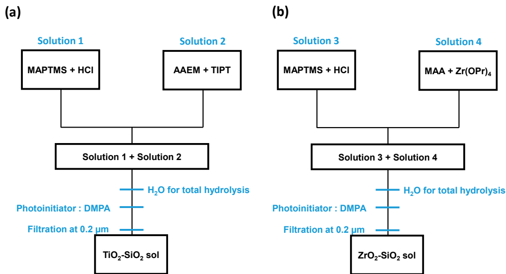
Figure 2. Preparation of the different organic–inorganic sol–gel solutions. Material synthesis of (a) TiO 2 –SiO 2 and (b) ZrO 2 –SiO 2 sols. In both cases, a photoinitiator (DMPA) is added to induce the start of UV-polymerization reactions.
