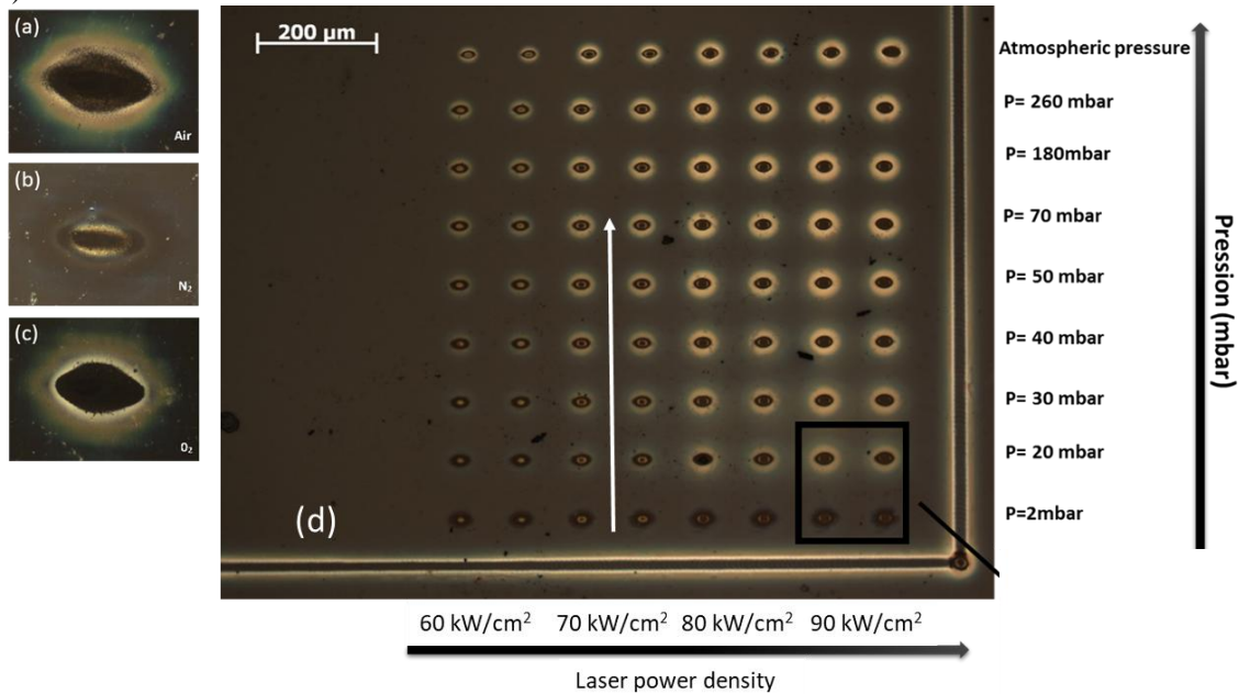
Figure 1 : pictures of laser spots written at 244 nm ( \tau = 1 \text{ s} ): (a) Air ( P_{\text{atm}} ), (b) N 2 ( P_{\text{atm}} ), (c) O 2 ( P_{\text{atm}} ). (d) increasing air pressures and laser power densities.
